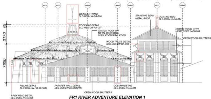
FR1 RIVER ADVENTURE ELEVATION 1
