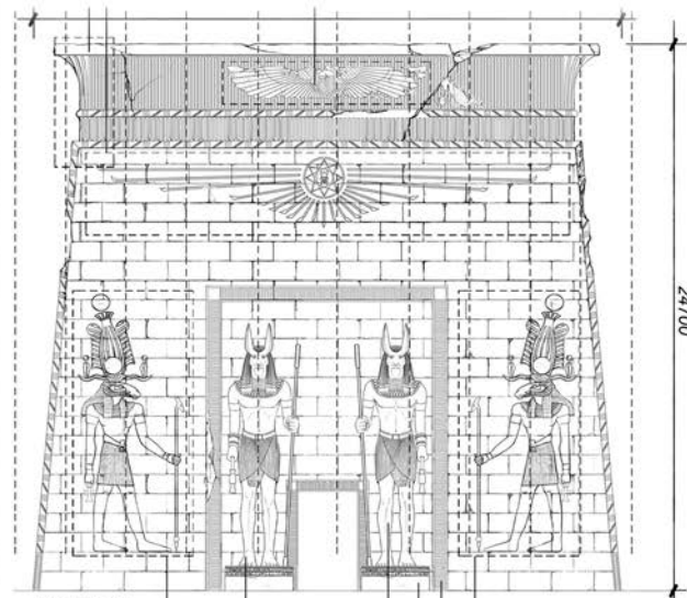
EXIT RIDE EXPLODED ELEVATION 2
